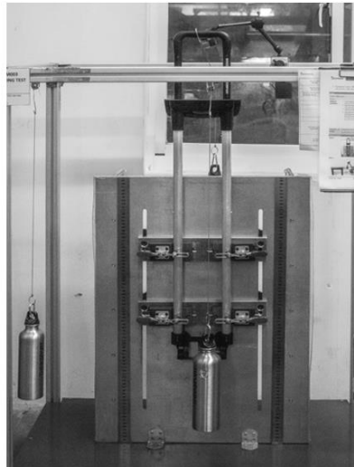
HANDLE WOGGLING TEST
