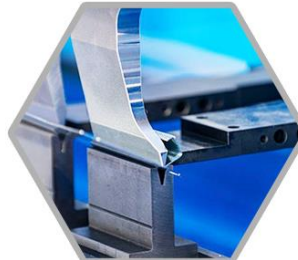
3D BENDING MACHINE
